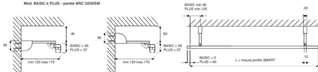
Mod. BASIC e PLUS - parete ARC 3230/SM
