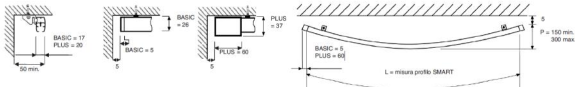
Mod. BASIC e PLUS - soffitto curve laterali
