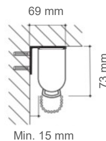
A parete Art 8650 + Art.8633
