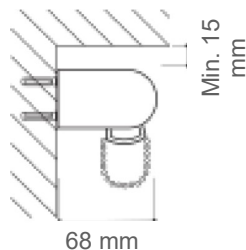
A parete Art.8601K
